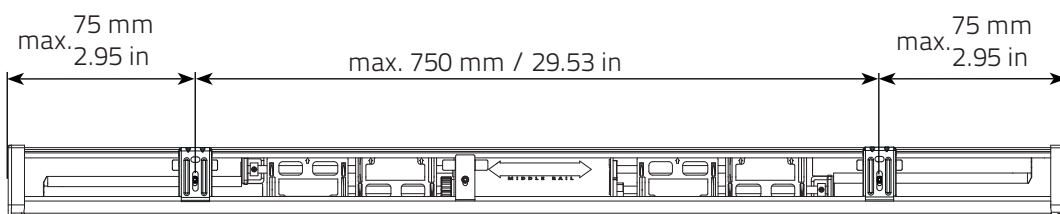
Inside mount
